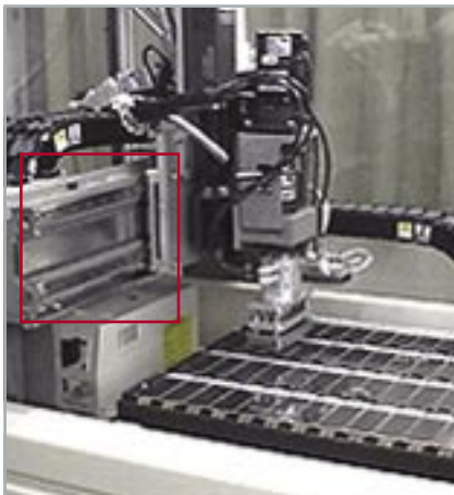
Application of Linear Motor Actuator (Medical instruments)
